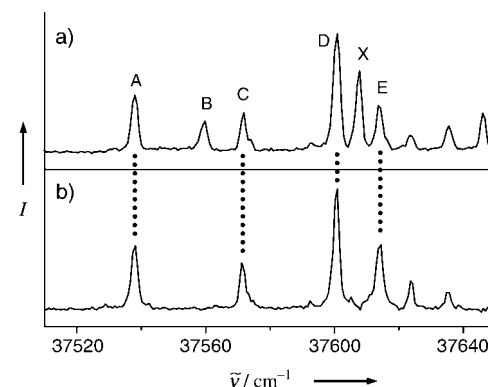
Figure 2. Mass-resolved R2PI excitation spectra of jet-cooled Phe obtained by a) one-color and b) two-color ionization. The wavelength of the ionization laser was fixed at 285.5 nm in (b).
